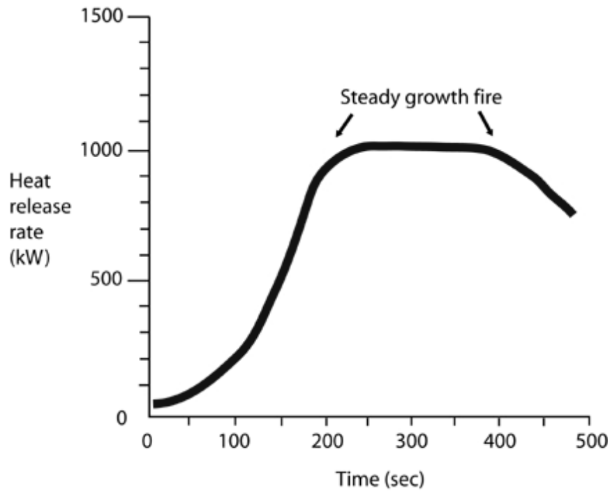
Figure 2-4 Graph of a Growing and Steady State Fire
